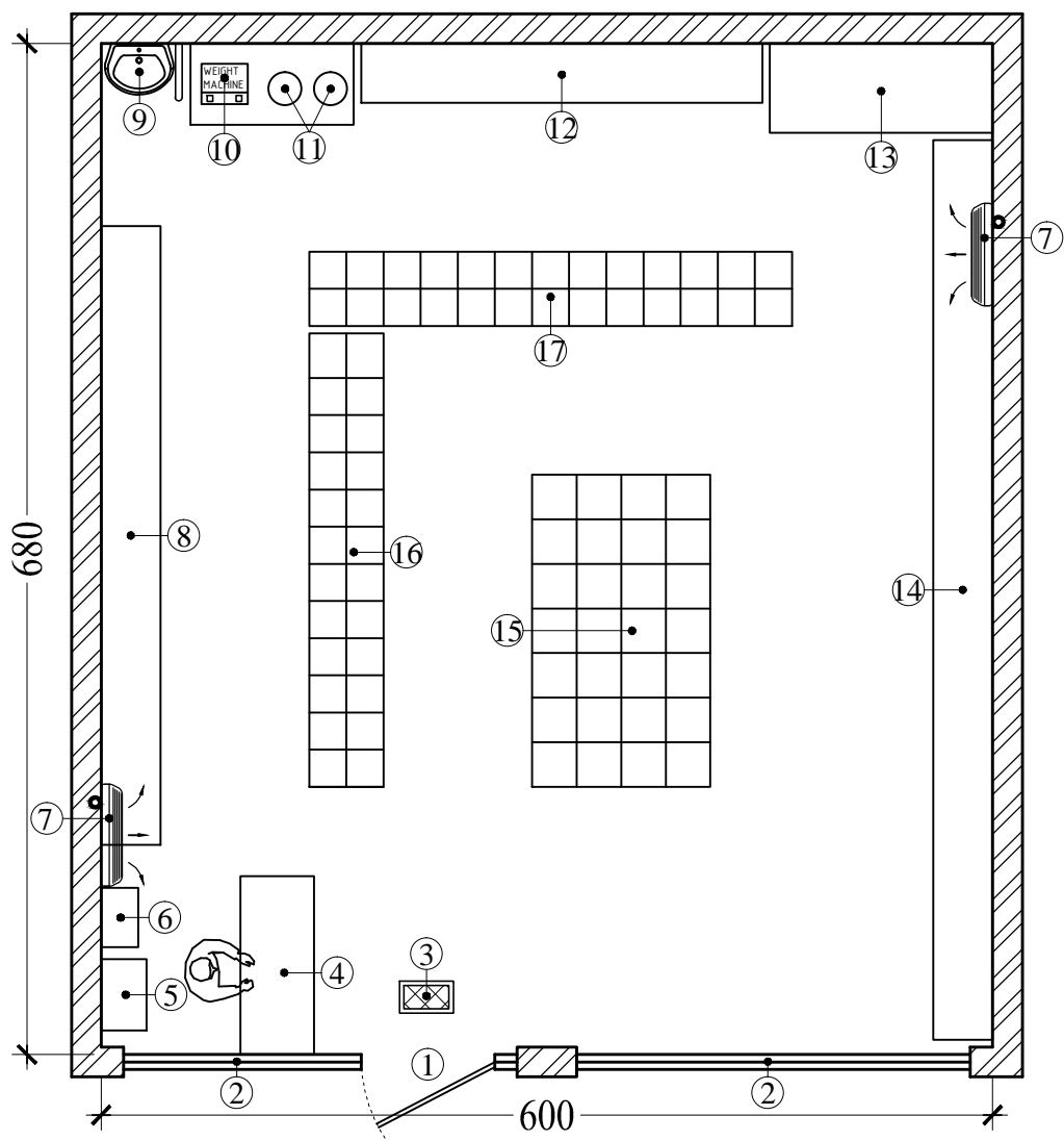
MODEL & STANDARD DESIGN OF ROASTERY
