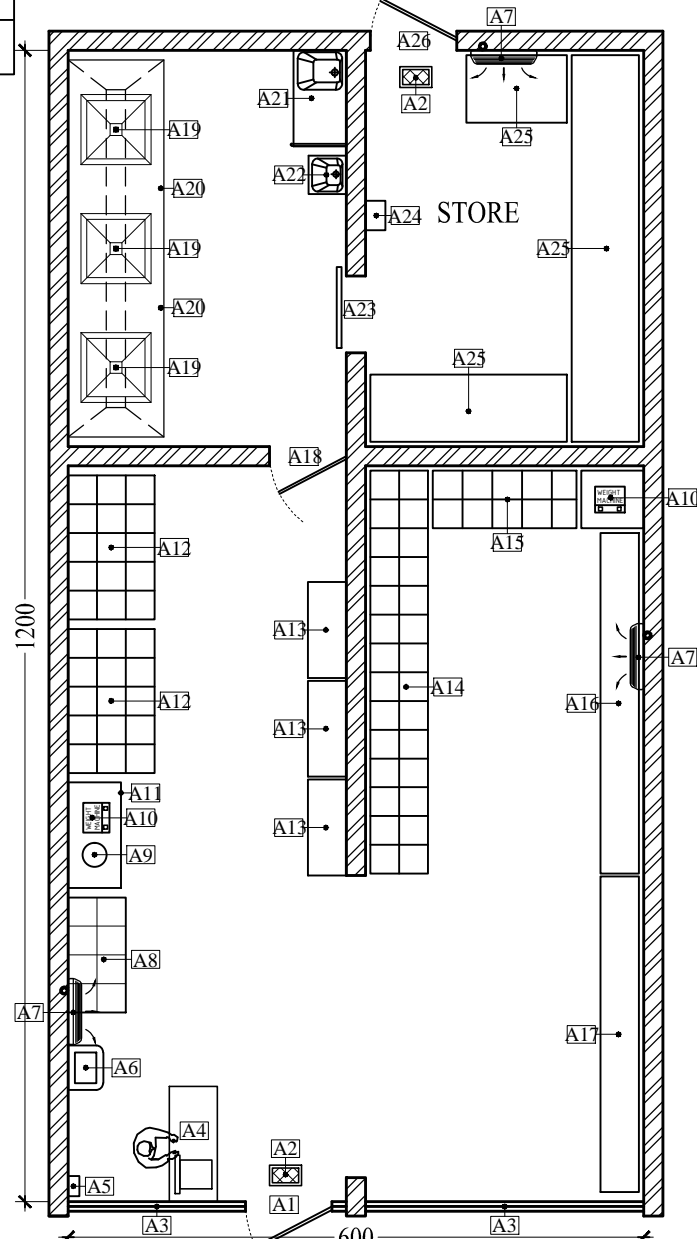
MODEL & STANDARD DESIGN OF FLOUR MILL & ROASTERY
