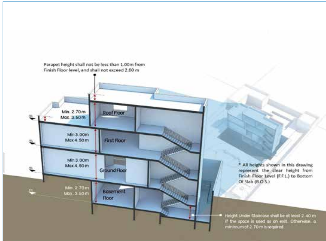
Figure 4: Net floor heights for residential villa.
