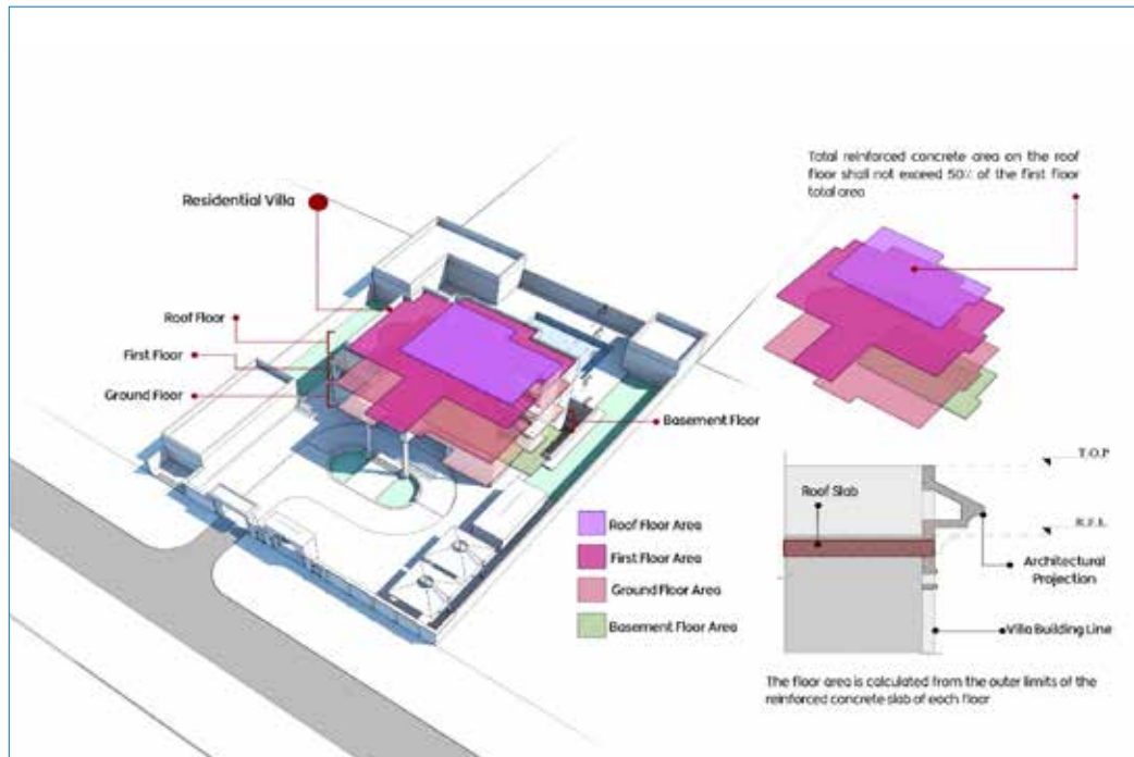
Figure 6: Roof floor permitted area
