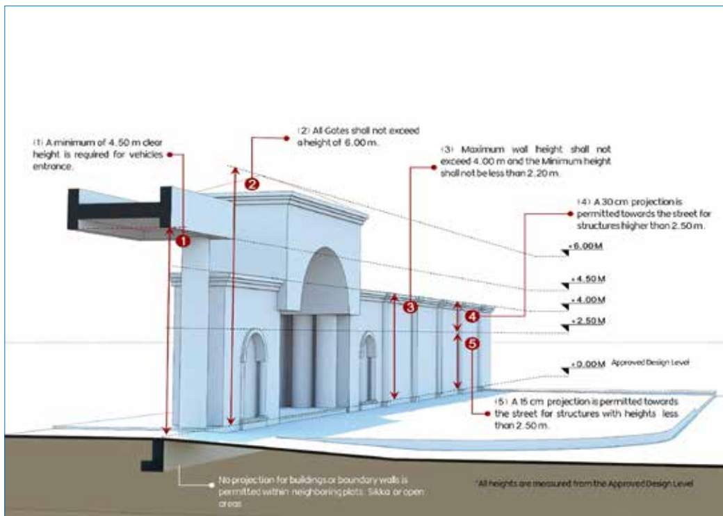
Figure 7: Residential Villa's Boundary Wall Requirements
