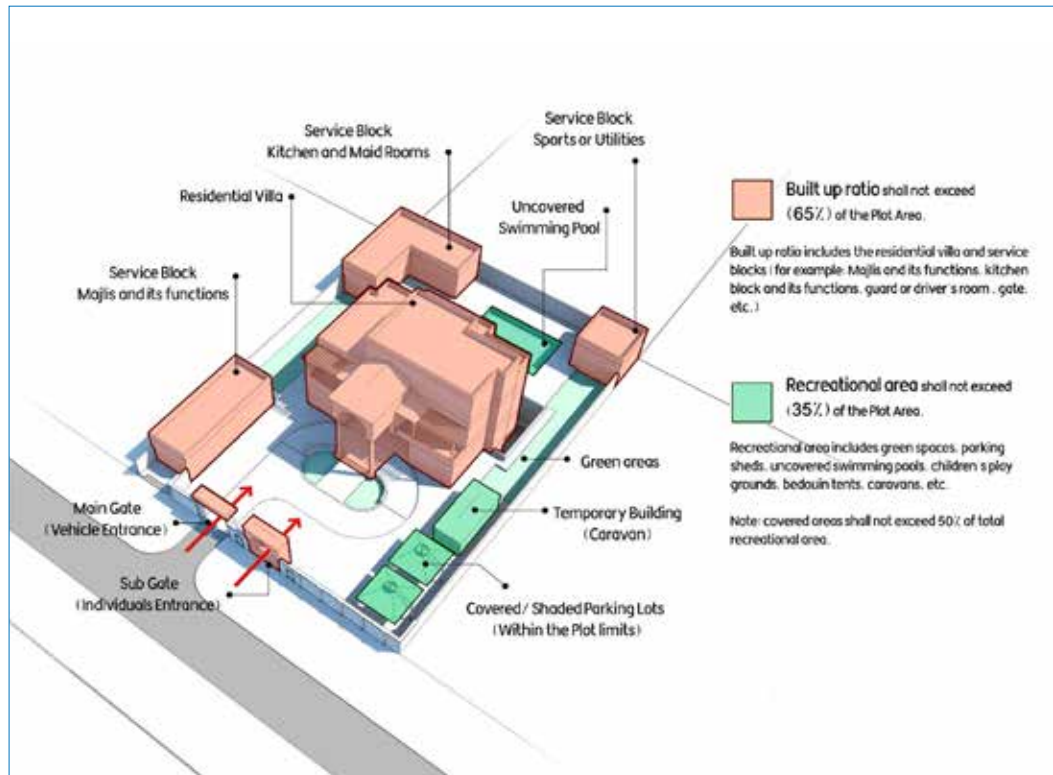
Figure 2: Built up Ratio of the Private Housing Plot
