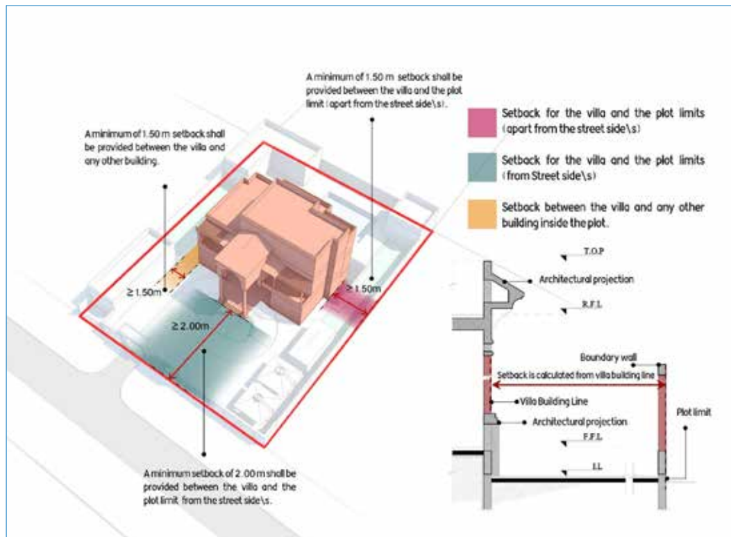
Figure 3: Setbacks of Residential Villas
