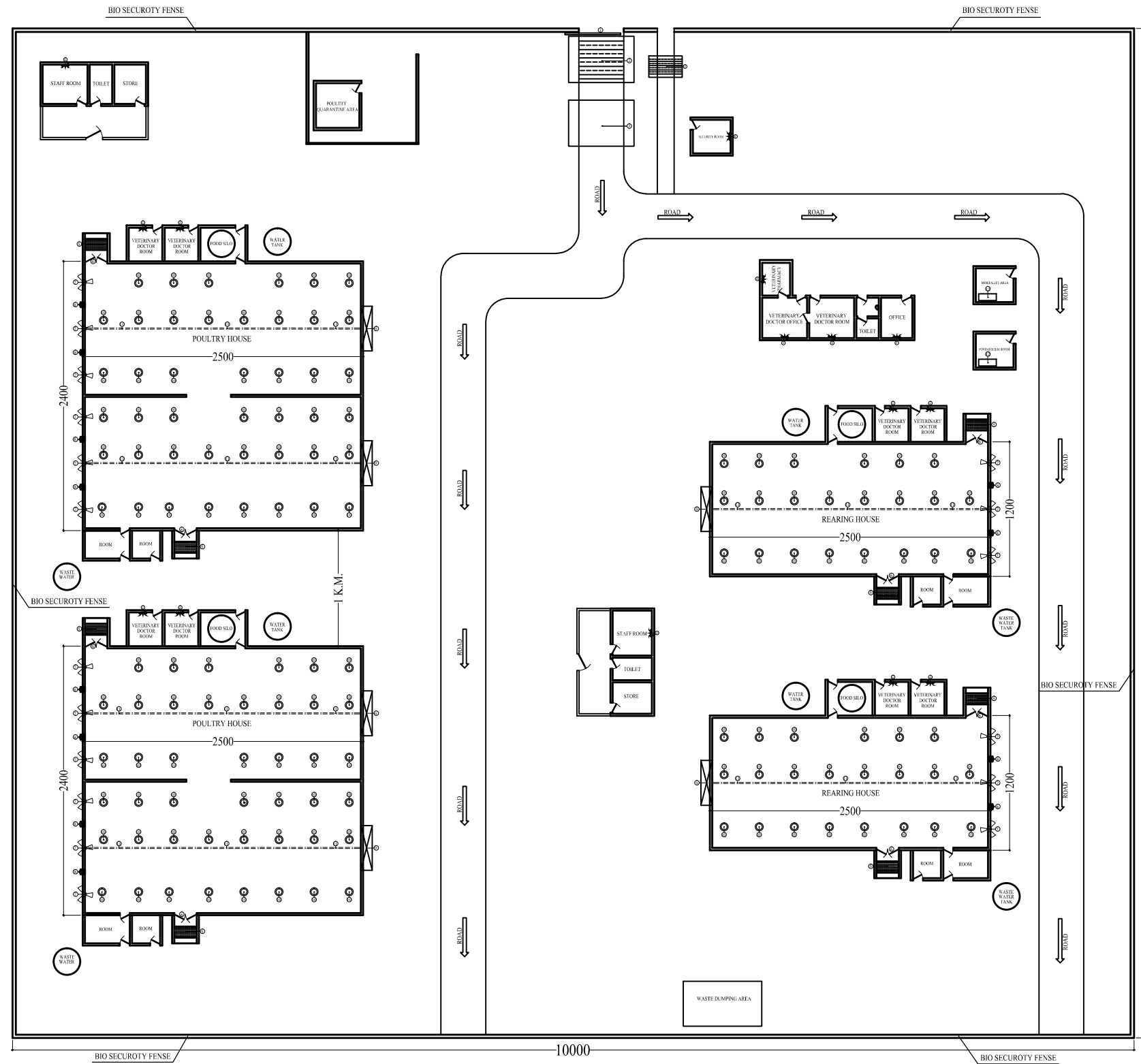
MODEL LAYOUT FOR POULTRY FARM
