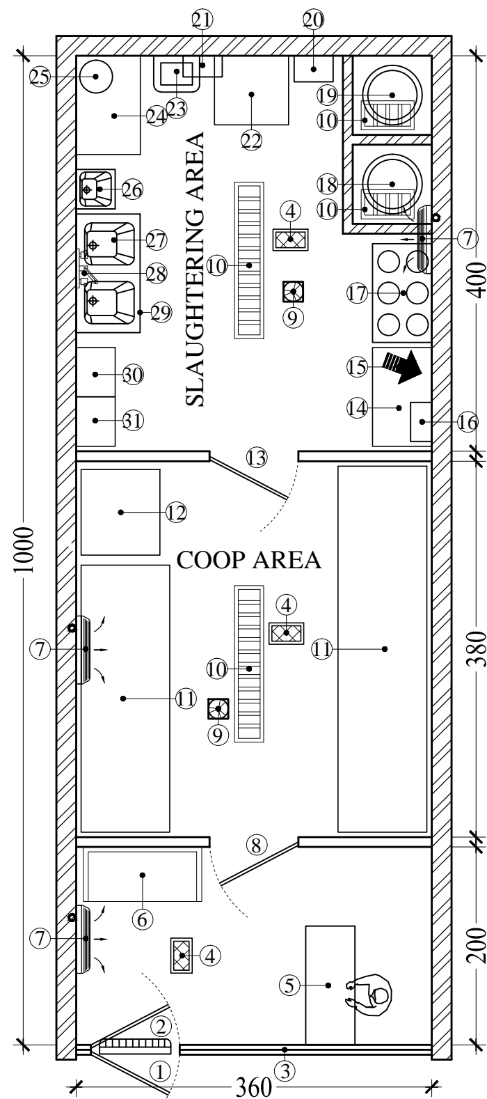
MODEL LAYOUT FOR LIVE POULTRY SLAUGHTERING
