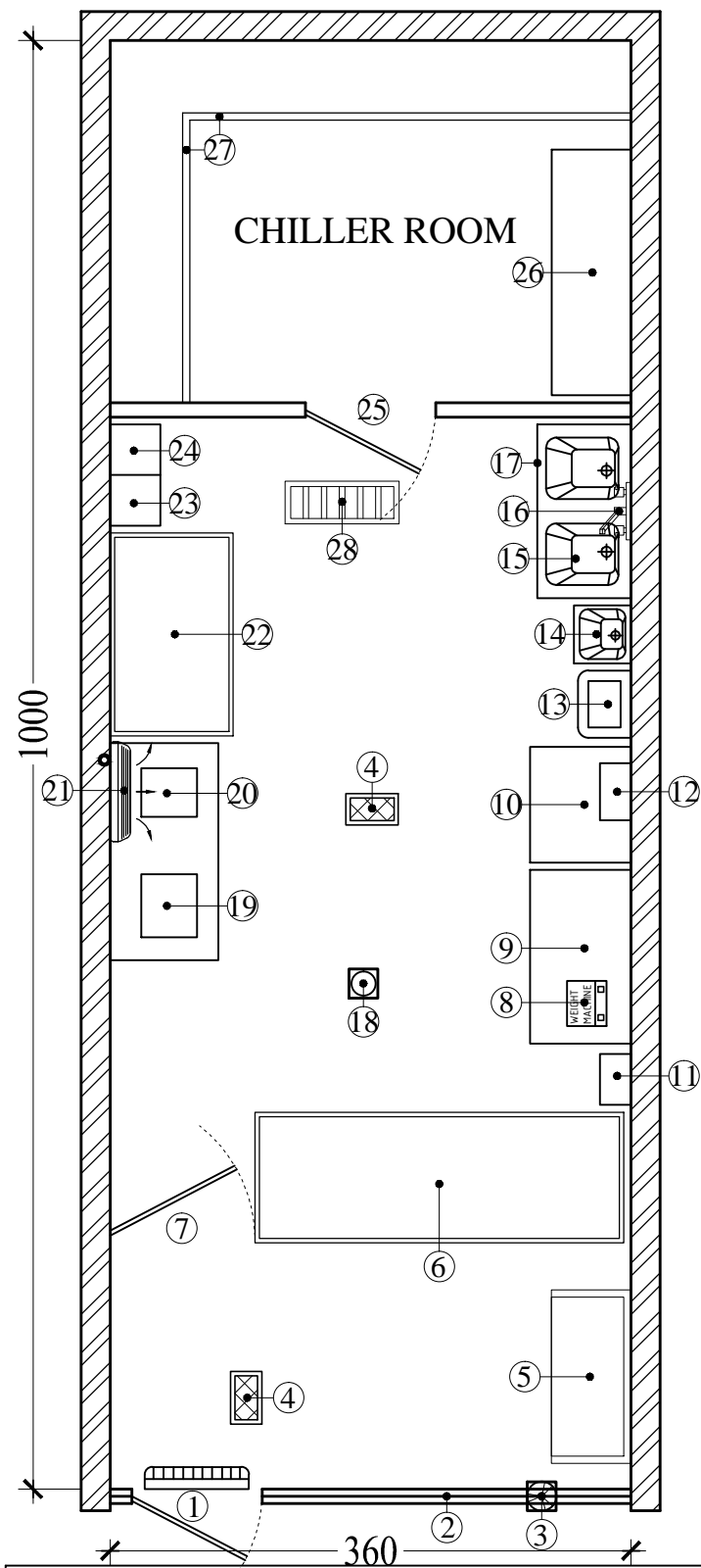
MODEL LAYOUT FOR BUTCHERY (RETAIL SALE OF FRESH MEAT)
