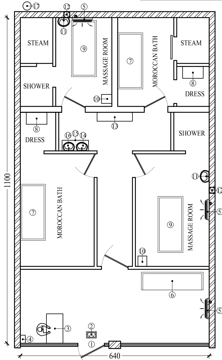
MODEL & STANDARD DESIGN OF SPA & ORIENTAL BATH
