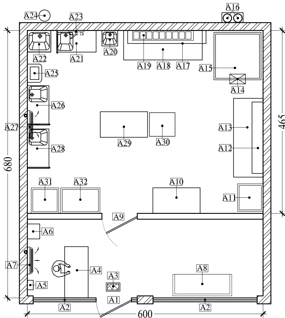
MODEL & STANDARD DESIGN OF FATAYER & MUAJANATH
